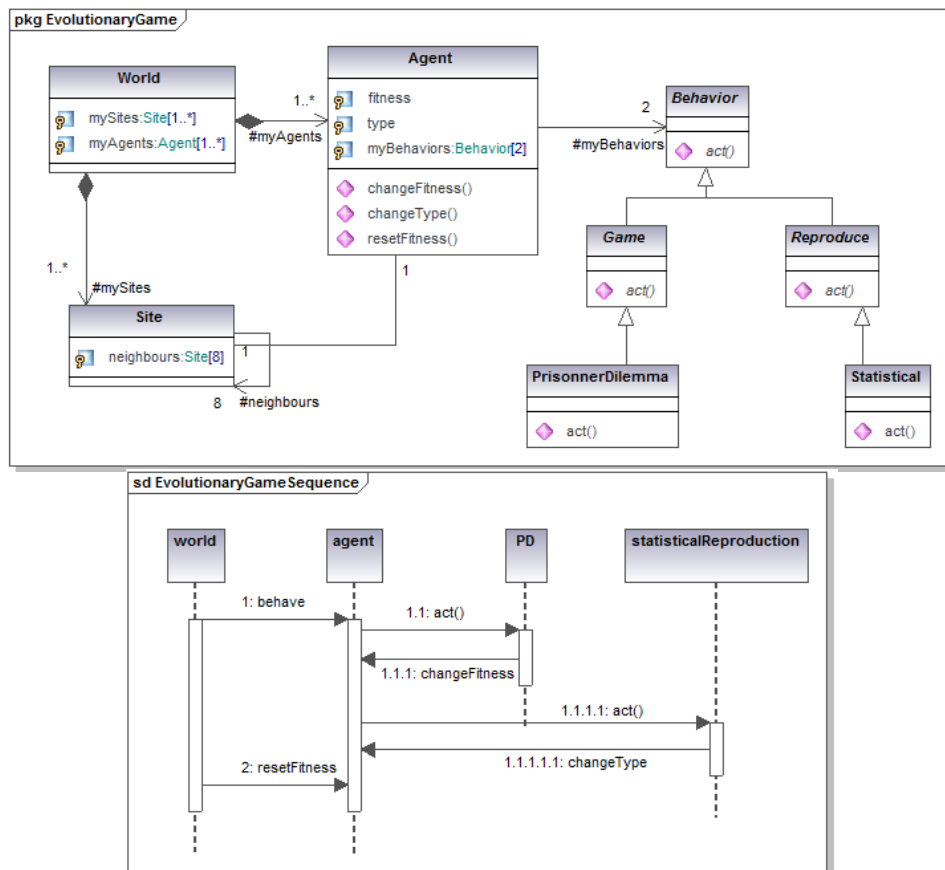
Figure 11. Spatial evolutionary game simulation class and sequence diagrams
