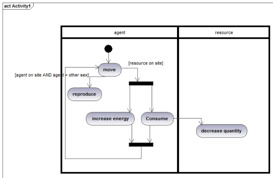
Figure 7. An activity diagram representing the same kind of situation as represented in the previous state diagram
