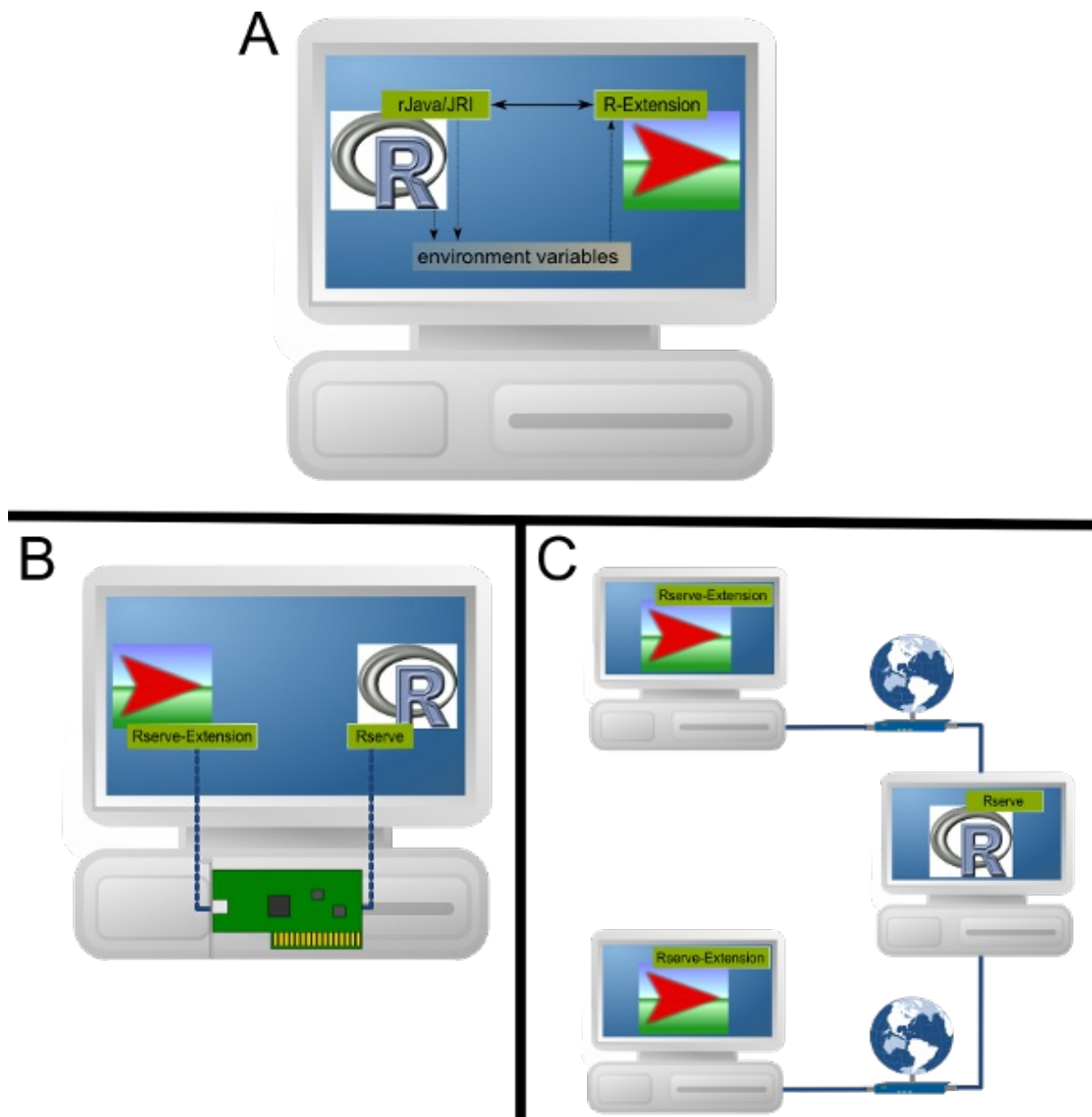
Figure 2. Communication of NetLogo's R- and Rserve-Extension with R. For the R-Extension, NetLogo uses the extension to communicate directly with R's rJava package (A). The R-Extension locates R and the rJava/JRI package by using environment variables of the operating system. For the Rserve-Extension, NetLogo uses a local network connection to communicate to an Rserve server running locally on the same machine (B) or one or multiple NetLogo clients use the Rserve-Extension to connect to a remote Rserve server via a network connection (C).
