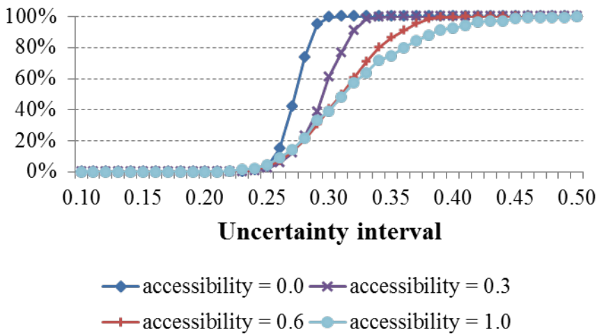
(c) Number of clusters = 3
