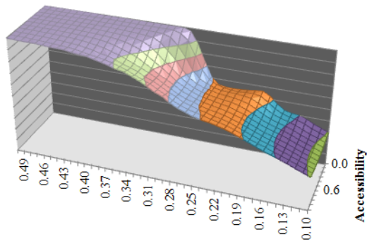
Figure 4. Size of the largest cluster (a) as a function of uncertainty interval and accessibility, (b) as a function of accessibility and connectivity.
