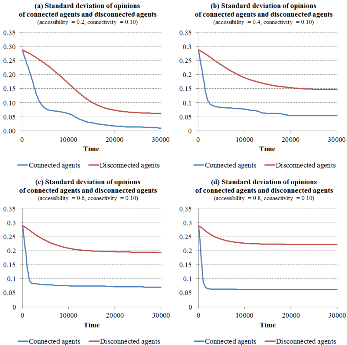
Figure 8. Standard deviation of opinions of connected agents and disconnected agents ( \mu = 0.3 , N = 1000 ) with (a) accessibility = 0.2, (b) accessibility = 0.4, (c) accessibility = 0.6, and (d) accessibility = 0.8. Standard deviation of connected agents' opinions decreases faster than standard deviation of disconnected agents' opinions.
