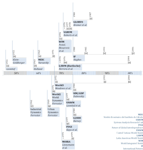
Figure 1. Timeline for a selection of global models and publications influential in the discipline. Vertical lines | : Approximate earliest activity of the project. Horizontal lines – : Citations related to the same project. Acronyms in bold: Global Model. Names in italic : Main researcher/author/project director. Asterisks (*): First report presented at IIASA (source: Meadows et al. (1982)).
