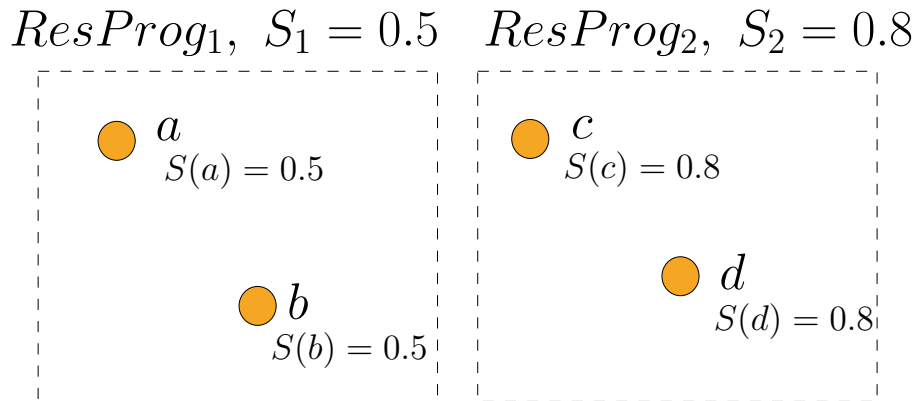
Figure 4: View V_1^0 of the debate for agent 1 at the start of the simulation.
