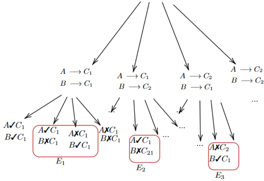
Figure 11: Representation of the probability tree.
