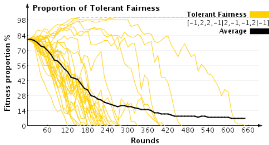
Figure 4: Tolerant Fairness playing against Defection
