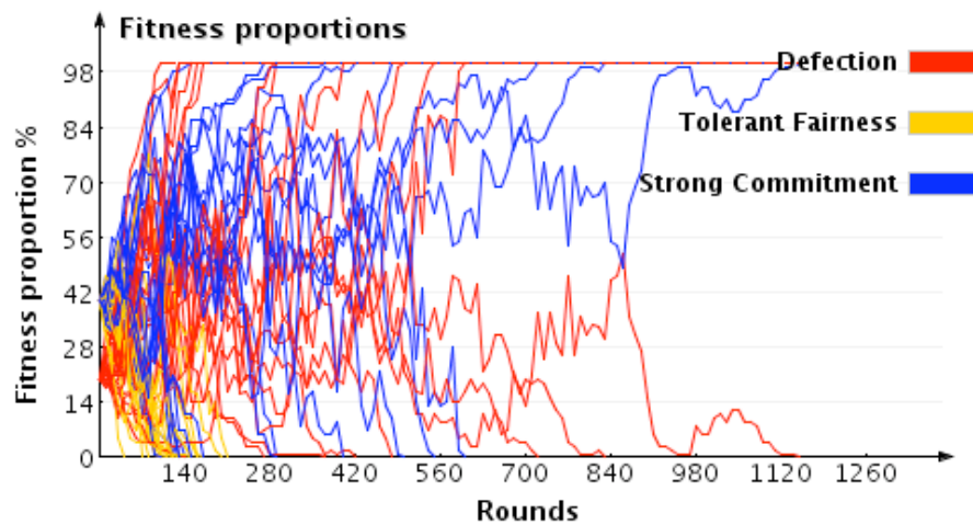
Figure 7: Fairness and Commitment playing against Defectors
