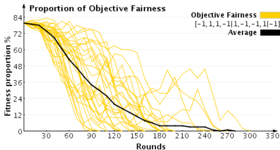
Figure 3: Objective Fairness playing against Defection
