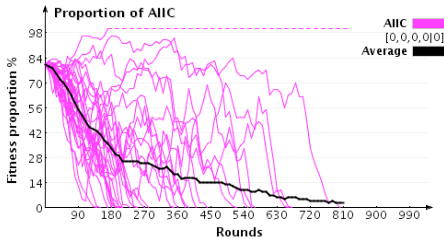
Figure 2: AIIIC playing against Defection
