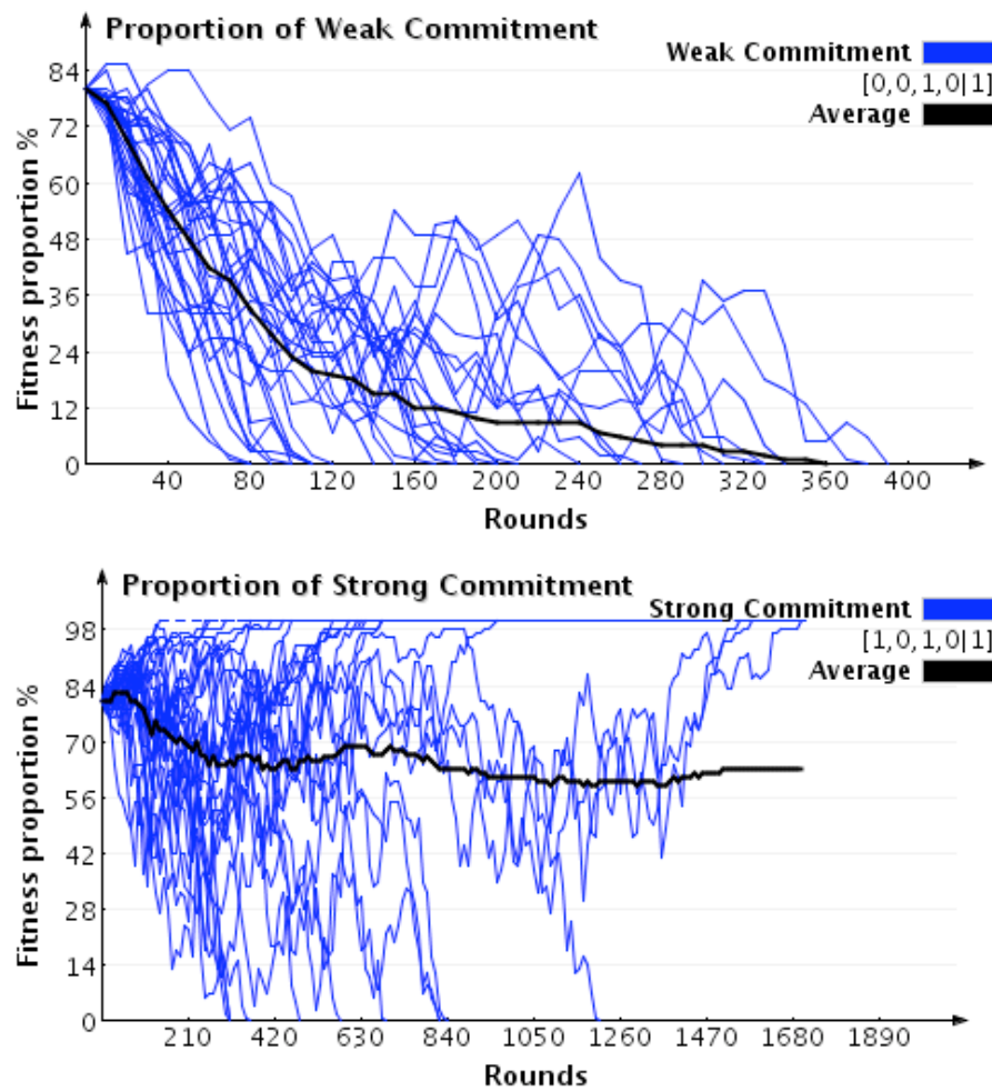
Figure 1: Weak and Strong Commitment playing against Defection
